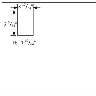
LED DRIVER
