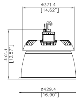
ALUMINUM REFLECTOR
