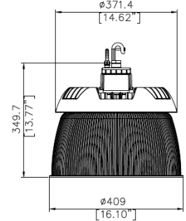
PRISMATIC REFLECTOR
