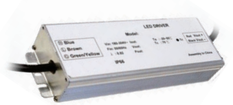
External Driver
